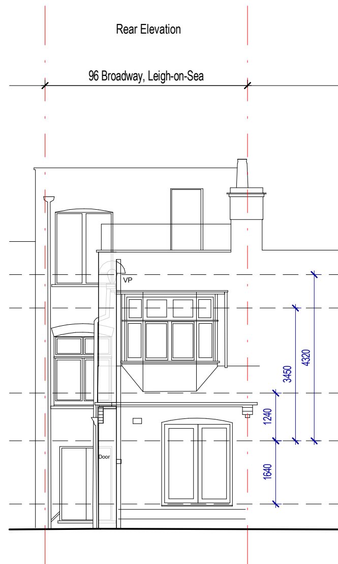
2 Rear Elevation PP102 1 : 100
